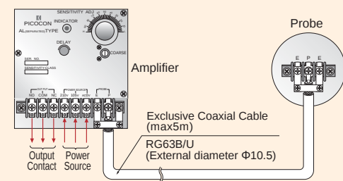
Wiring Diagram
